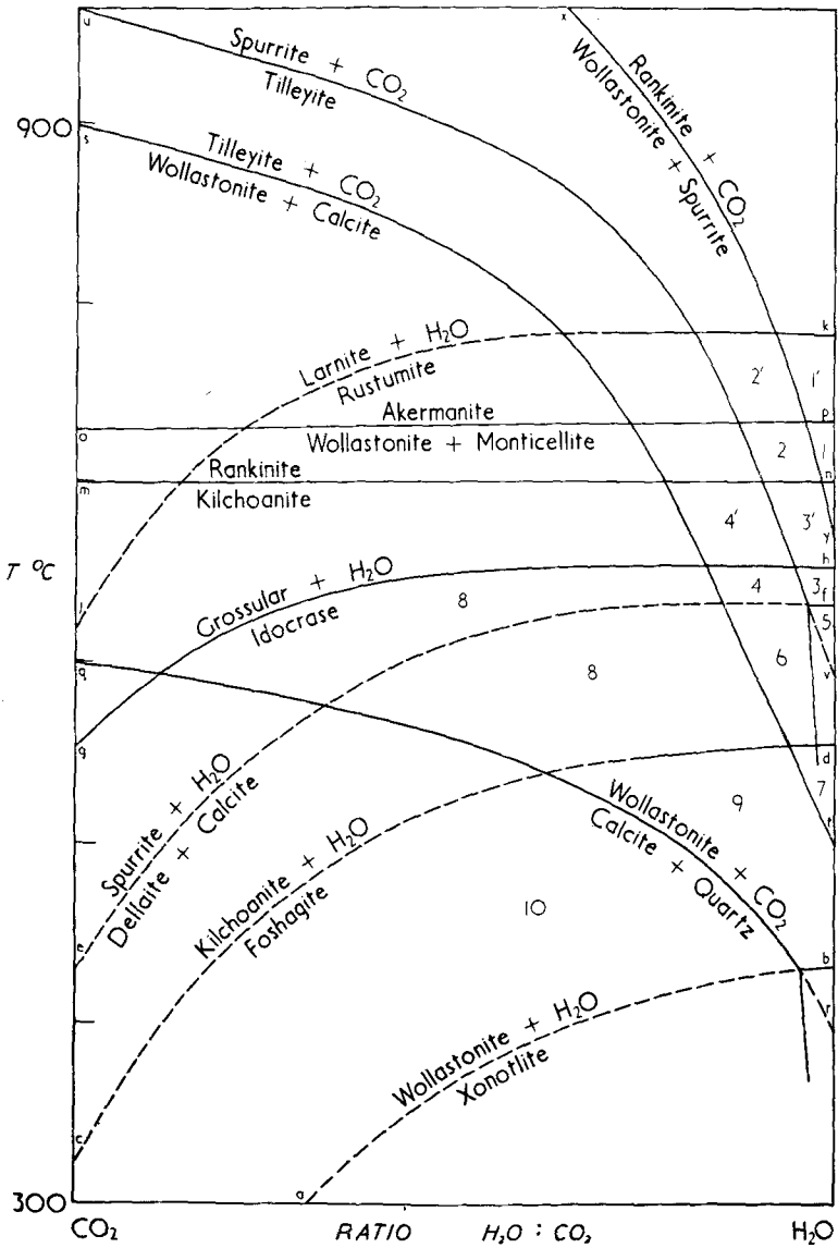
FIG. 1. An isobaric plot of temperature against the ratio of \text{CO}_2 : \text{H}_2\text{O} in the vapour phase, assuming P(\text{H}_2\text{O} + \text{CO}_2) = P(\text{load}) . This illustrates schematically the stability fields of some of the minerals in the metamorphosed limestones at Kilchoan.
