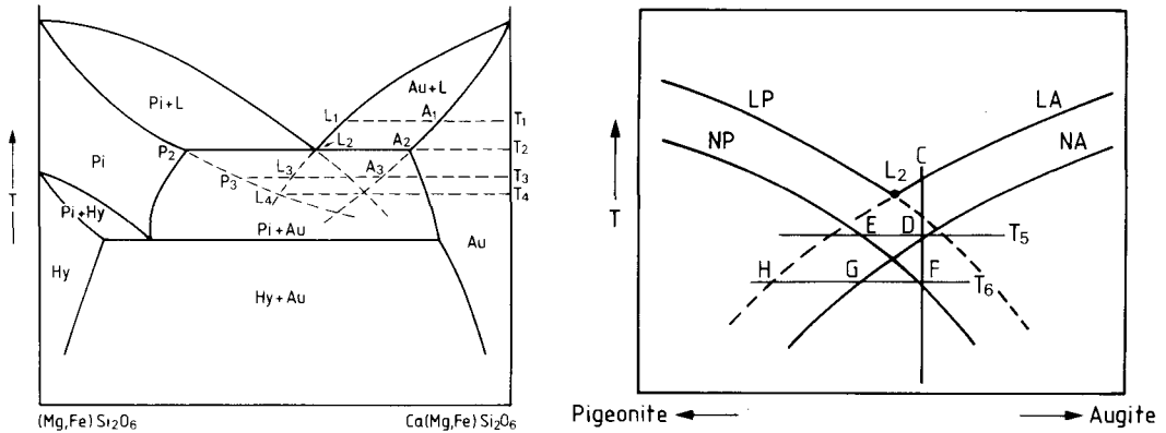
Fig. 3 (a, left). Hypothetical pseudobinary phase diagram to model crystallization of pyroxenes from tholeiitic magmas under metastable conditions. For details of sequences see text. (b, right). Enlargement of central part of liquidus curves of fig. 3a to show effects of supersaturated crystallization under nearly isothermal conditions. LA liquidus augite, LP liquidus pigeonite, NA nucleation curve augite, NP nucleation curve pigeonite. Crystallization sequences for T5 and T6 are discussed in the text.
