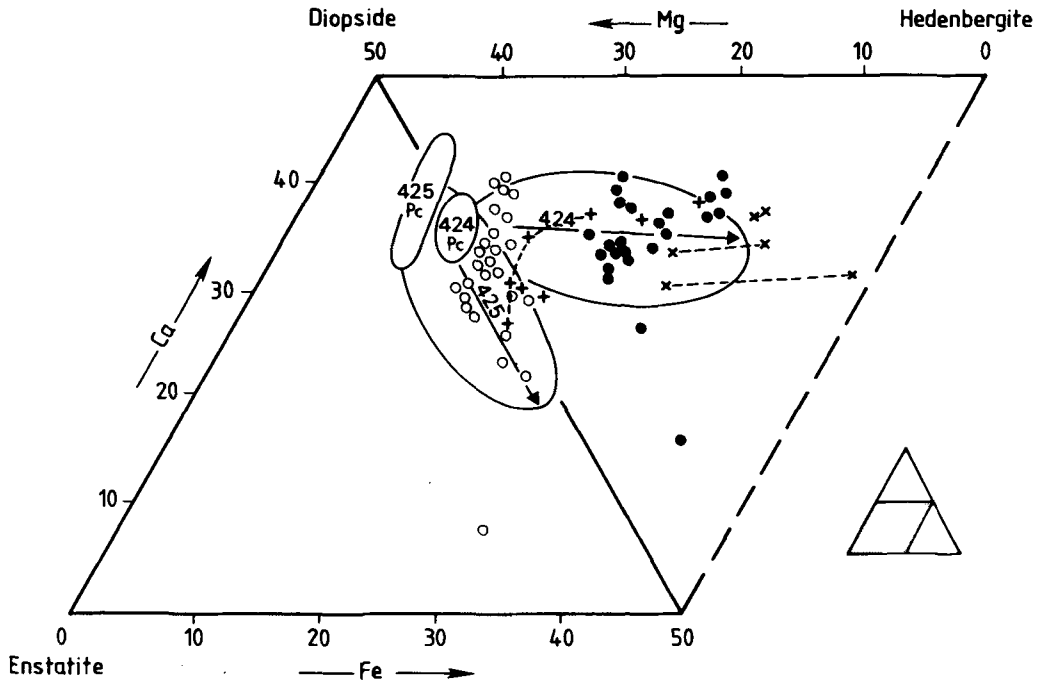
FIG. 2. 425Pc and 424Pc, range of phenocryst compositions encountered at GSC Sites 425 and 424 respectively. Arrows show generalized fractionation trends for groundmass pyroxenes for which limits of variation are indicated by elliptical areas. Also shown are groundmass pyroxenes from Section 424-6-1 (piece 10): closed circles, granular pyroxenes of mesostasis; open circles, ophitic grains; crosses, feathery extensions of ophitic pyroxenes extending into Fe-rich formerly glassy regions. Dotted lines link analyses from same crystal and indicate how clinopyroxenes become enriched in Fe and Ca as they grow into glassy regions (after Matthey and Muir, 1980, but with additional data).
