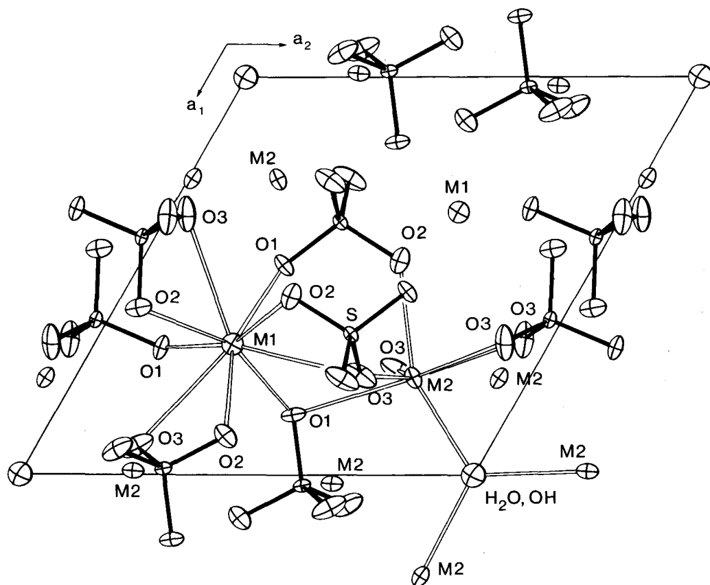
FIG. 1. ORTEP plot (Johnson, 1965) of the crystal structure of cesanite. The section plane is nearly parallel to (110). The M(1) site is occupied by Na, the M(2) site by Na + Ca.
