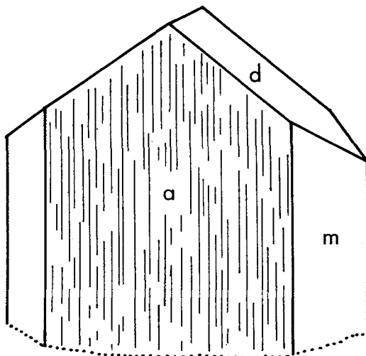
FIG. 1. Obradovite; crystals are slightly elongated along c and {100} faces are striated in the c direction.
