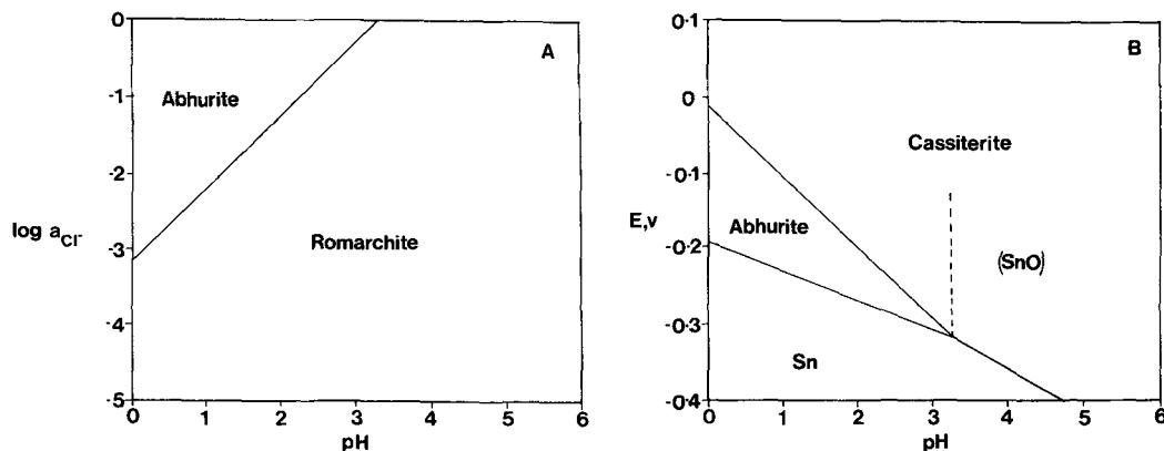
FIG. 1. (a) Stability field diagram for the \text{SnO-HCl-H}_2\text{O} system at 298.2 K and 10^5\text{Pa} ; (b) Potential-pH diagram for the \text{Sn-H}_2\text{O-HCl} system at a_{\text{Cl}^-} = 1 . The limit of stability of abhurite with respect to \text{SnO} is shown by the dashed line.
