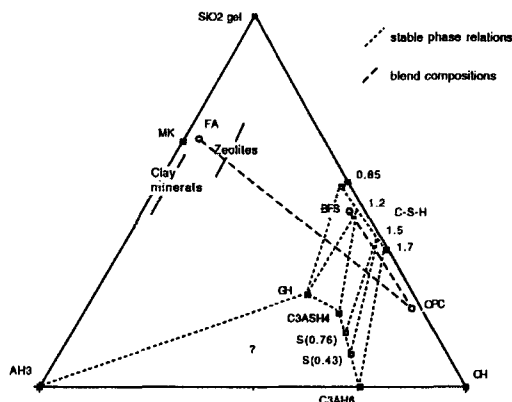
FIG. 1. Phase relations in the water-saturated portion of the C-A-S system at 25°C: CEMCHAM 1, in relation to cement blends (mol%). Approximate composition ranges for zeolites and clays are also shown.
