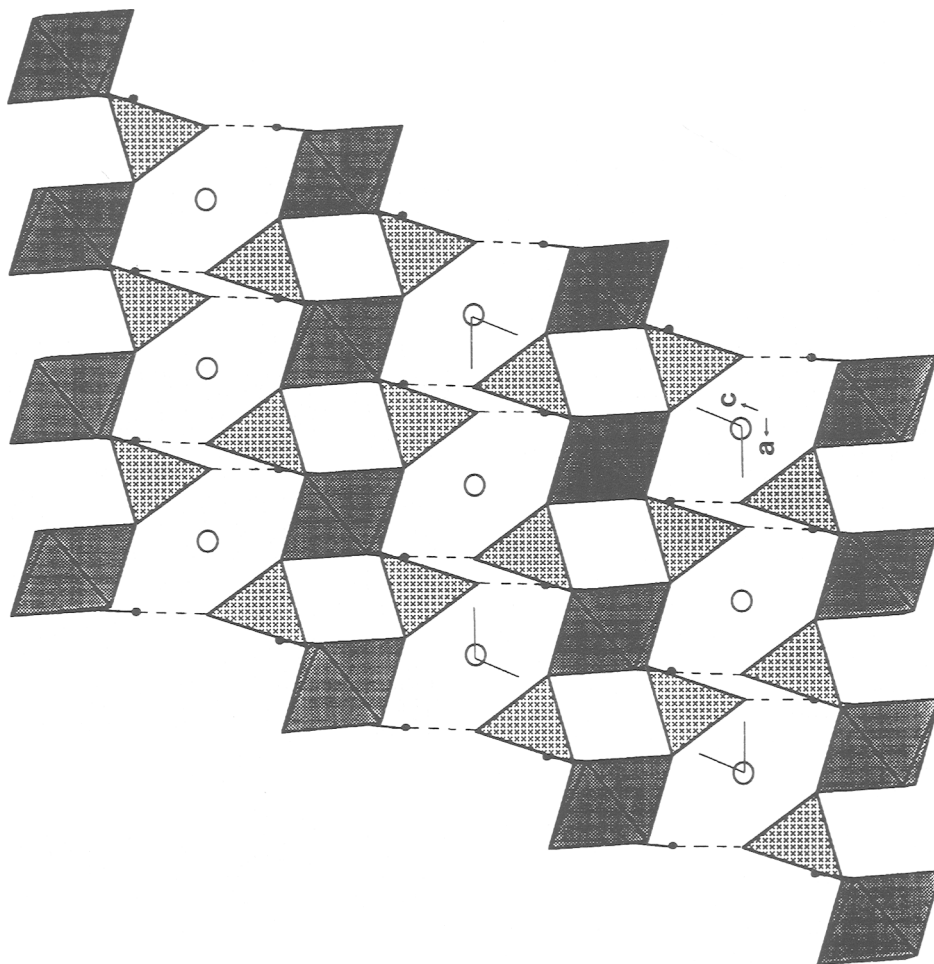
FIG. 2. Schematic diagram of the mawbyite structure down [010] showing the polyhedral likages and the proposed hydrogen bonding network. The Pb atoms are shown as open circles.
