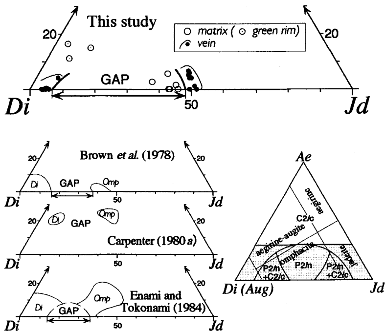
FIG. 3. Chemical compositions of the clinopyroxenes in the omphacitite block from the Osayama serpentinite melange plotted on a jadeite (Jd)-aegirine (Ae)-diopside (Di) ternary diagram. The compositional ranges reported by Brown et al. (1978), Carpenter (1980a) and Enami and Tokonami (1984) are also shown in small diagrams.
