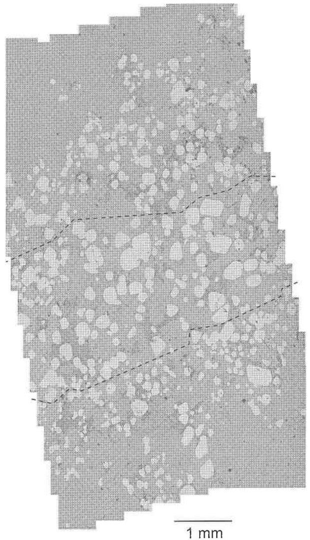
FIGURE 1. Photomosaic of digital backscattered electron images of a thin, symmetrically size-graded chromitite layer (sample F) from Gabbro-norite Zone I of the Lower Banded series of the Stillwater Complex, Montana. Chromite grains are shown as light-colored, equant grains. Undifferentiated silicate minerals (mainly plagioclase and pyroxene) compose the darker gray background. The layer generally extends from lower left to upper right. Dashed lines outline the central region of larger grains: CSD curves were determined on all grains in the layer and on grains in the central and marginal portions separately (Fig. 4).
