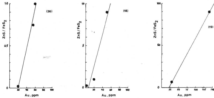
FIG. 15. A plot of gold concentration against sphalerite/pyrite ratio for mineral concentrates of differing mineral proportions produced from the same specimen.
