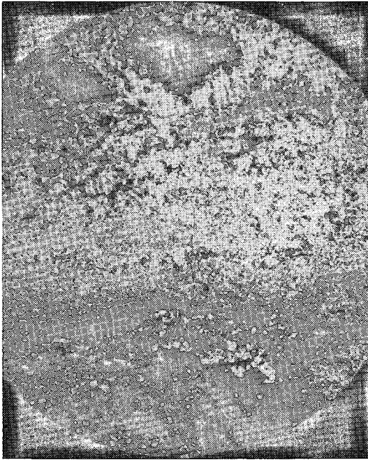
FIG. 4. Layered sulfides with a thick pyrite-sphalerite band characterized by a fine-grained, intimate mixture of minerals above a narrower band of massive sphalerite with a few large pyrite crystals. Field of view is 2.5 cm.
