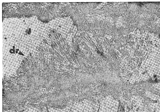
FIG. 5. Photomicrograph (transmitted light) of acicular dravite (dr) in a quartz + dravite vein that cuts across foliation of schist. Bar scale 25 \mu m.
