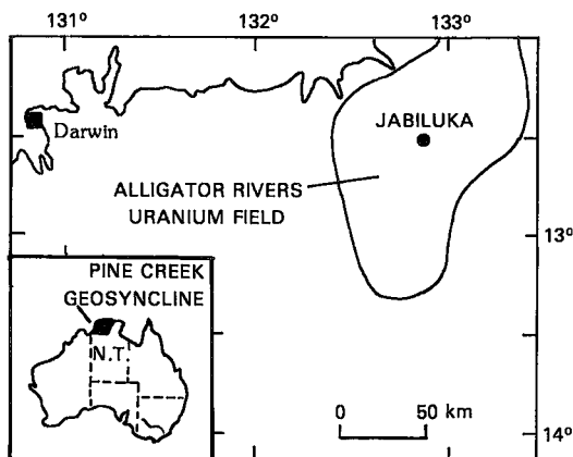
FIG. 1. Location of the Pine Creek geosyncline and the Alligator Rivers Uranium Field (ARUF) in northern Australia.
