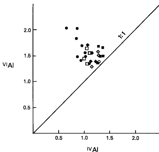
FIG. 11. Values of the ratio of ^{VI}Al to ^{IV}Al in the chlorites in metasedimentary rocks at Jabiluka. Clay-size chlorite shows by far the largest range in values. Symbols as in Figure 10.
