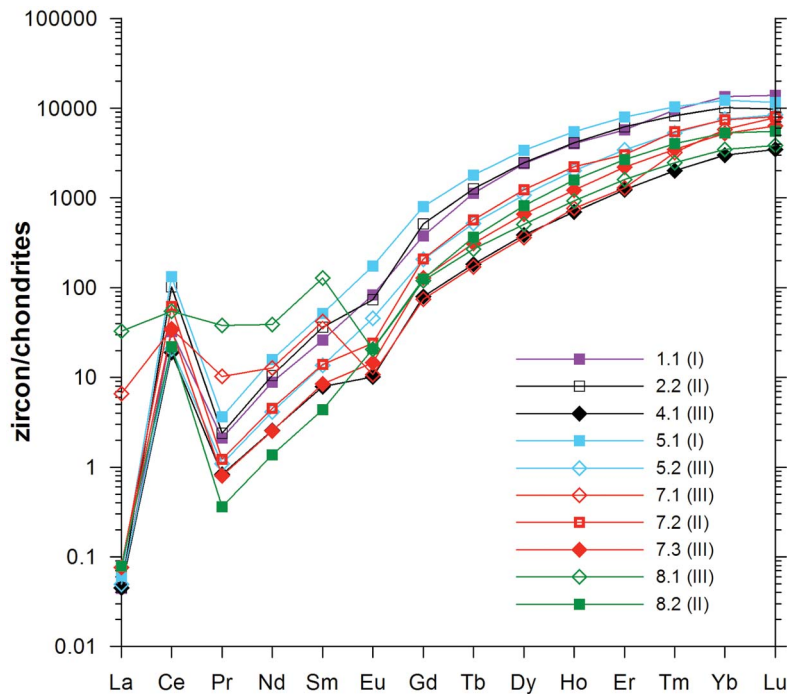
Fig. 7a. REE patterns of some spots of zircon crystals represented in Figure 4. Numerical data are given in Table 3, together with Hf and Y content of these zircon crystals. The textural type of the recrystallized areas is indicated in the legend for each spot by the Roman numeral (in parentheses), together with the number of the analysis.
