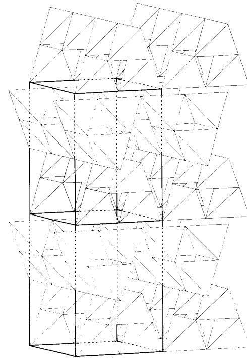
Fig. 5. View of the two-layer structure. The centers of the \text{Hg}_4\text{I}_{10} groups in neighboring layers are displaced by \frac{1}{2} (\mathbf{a} + \mathbf{b})
