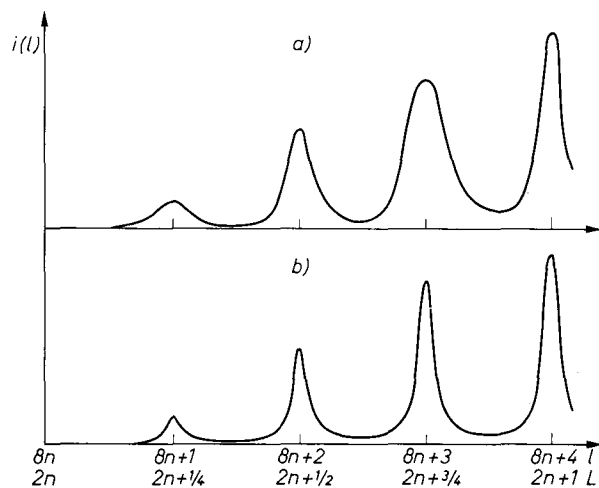
Fig.2. (a) Mean curve for i(l) = \frac{I(l)}{f_{\text{Hg}}^2} measured on a Weissenberg photograph of a very small disordered crystal along the streak 12l . The curve is periodic with a period of eight in l and symmetrical at l = 4n . (b) The theoretical curve calculated with s = 2 and \omega_1 = 1 - \omega_2 = 0.1 is shown for comparison
