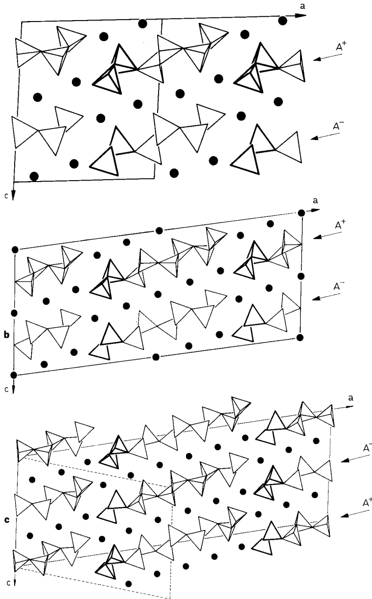
Fig. 1. Projection of the structure of the Ba silicates onto (010): a) \text{Ba}_4[\text{Si}_6\text{O}_{16}] , b) \text{Ba}_5[\text{Si}_8\text{O}_{21}] , c) \text{Ba}_6[\text{Si}_{10}\text{O}_{26}] . The length of the multiple chains is perpendicular to the plane of projection and their width is almost parallel to a . For illustration, one subchain of each multiple chain is outlined by heavy lines. The multiple chains have two orientations labelled A^+ and A^- ; they are joined by Ba atoms, indicated by black dots. In c) the dashed line indicates a primitive cell and the solid line a B-centered cell, the setting adopted in this paper
