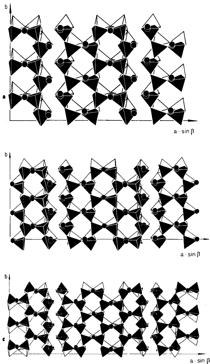
Fig. 2. Projections of the structures parallel to [001]: a) Ba_4[Si_6O_{16}] , b) Ba_5[Si_8O_{21}] , c) Ba_6[Si_{10}O_{26}] . In contrast to the others, in Ba_5[Si_8O_{21}] the adjoining multiple chains in the [100] direction are shifted by b/2 relative to one another; this has the effect of producing a C-centered cell. The Ba atoms are positioned at the sides of interstices between the subchains, resulting in tunnels running through the structure. The anterior Ba atoms are positioned in front of the chains and the posterior Ba atoms between the chains
