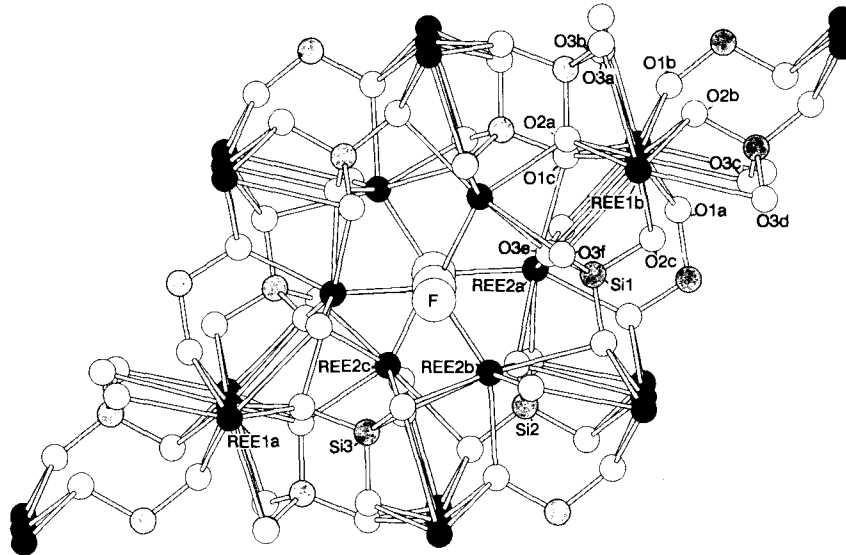
Fig. 1. Atomic arrangement of P2_1 britholite tilted 10^\circ from [001] .
