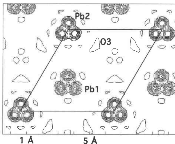
Fig. 2. Final electron-density map, \rho(x, y, \frac{1}{4}) , for plumboferrite. The contours drawn correspond to 2, 4, 6, 10, 20, . . . , 80 e^-/\text{Å}^3 . The origin of the unit cell is at the upper left corner, with x downward and y horizontal.
