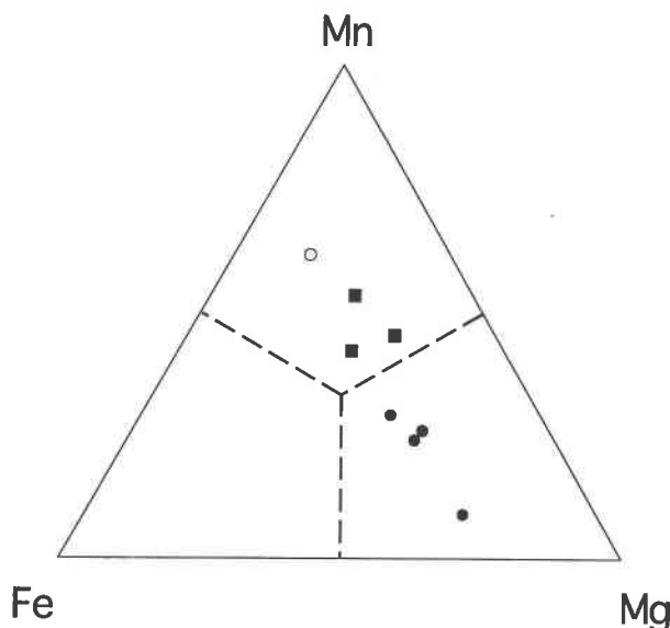
Fig. 1. Triangular plot of the system (\text{Mg}, \text{Mn}, \text{Fe}^{2+})\text{Fe}_2\text{O}_4 showing the composition of spinels. Solid circles, squares, and the open circle refer to pure plumboferrite samples, plumboferrite-lindqvistite pairs, and pure lindqvistite samples, respectively. Two of the data points are taken from Holtstam and Norrestam (1993); the others are from this work.
