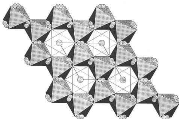
FIGURE 1. Crystal structure of phase D projected along c . Shaded and unshaded octahedra represent \text{SiO}_6 and \text{MgO}_6 octahedra, respectively. Large spheres represent Mg and small ones H.
