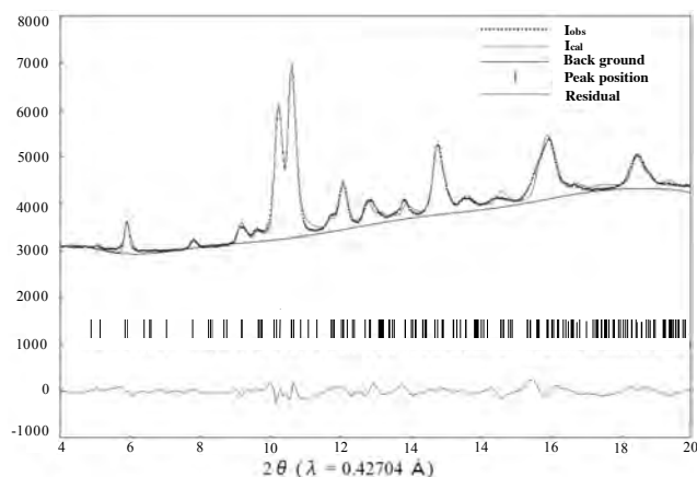
FIGURE 8. Rietveld profile fitting of the new high-pressure phase of \text{CaFe}_2\text{O}_4 . The diffraction pattern was taken at 63.3 GPa.
