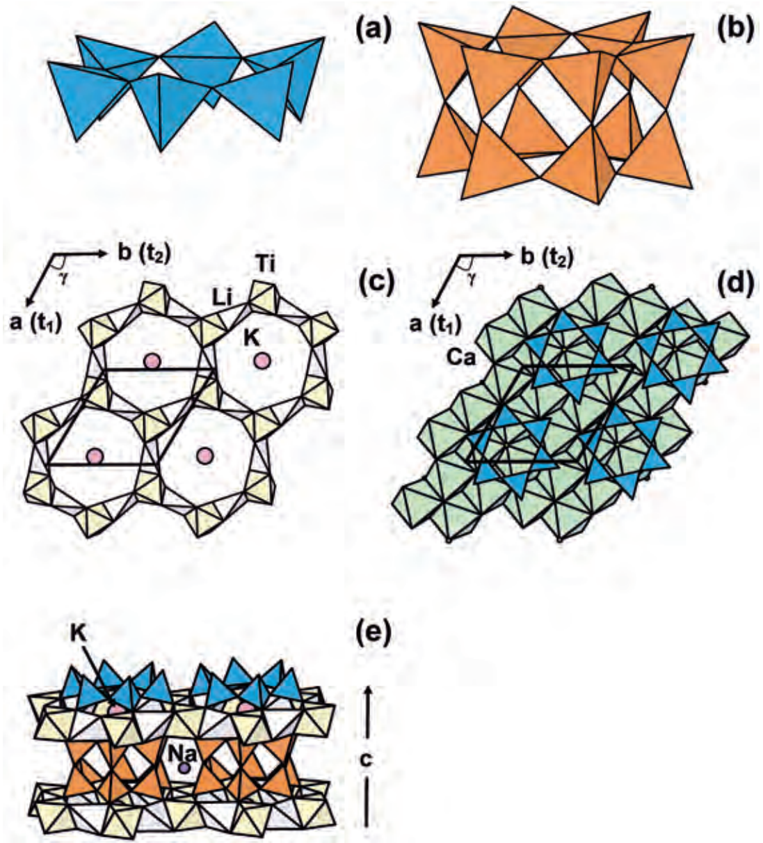
FIG. 1. Fragments of the crystal structure of faizievite: (a) a six-membered single beryl ring [ \text{Si}_6\text{O}_{18} ]; (b) a six-membered double milarite ring [ \text{Si}_{12}\text{O}_{30} ]; (c) a sheet of (\text{LiO}_4) tetrahedra and (\text{TiO}_6) octahedra and K atoms in large voids viewed down [001] ; (d) a sheet of Ca-dominant M(1,2,3,4) octahedra and adjacent [ \text{Si}_6\text{O}_{18} ] rings viewed down [001] ; (e) linkage of (\text{Si}_{12}\text{O}_{30}) and (\text{Si}_6\text{O}_{18}) rings and a sheet of (\text{LiO}_4) tetrahedra and (\text{TiO}_6) octahedra viewed down [110] . The (\text{SiO}_4) tetrahedra of milarite and beryl rings are orange and blue, the (\text{LiO}_4) tetrahedra are grey, the (\text{TiO}_6) octahedra are honey yellow; the M(1,2,3,4) octahedra are green, A(1) (= Na), A(2) (= K) and F atoms are shown as large pink, medium purple and small yellow circles, respectively.
